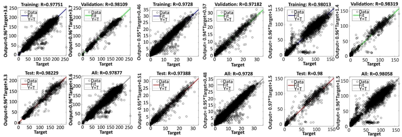
Figure 4. Prediction of electrical consumption power for Leaf Lab, Summa and Kite Lab from 1 May 2017 to 1 August 2017.
